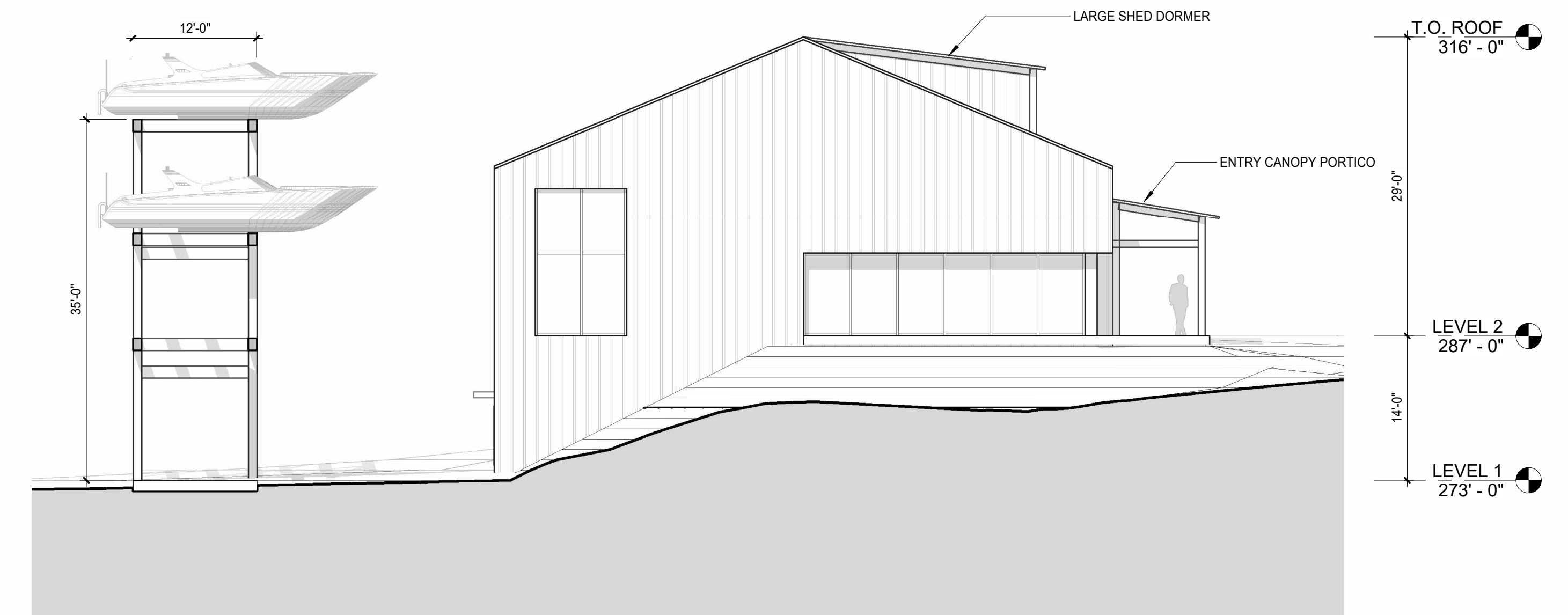
④ Southeast Elevation 1" = 10'-0"
