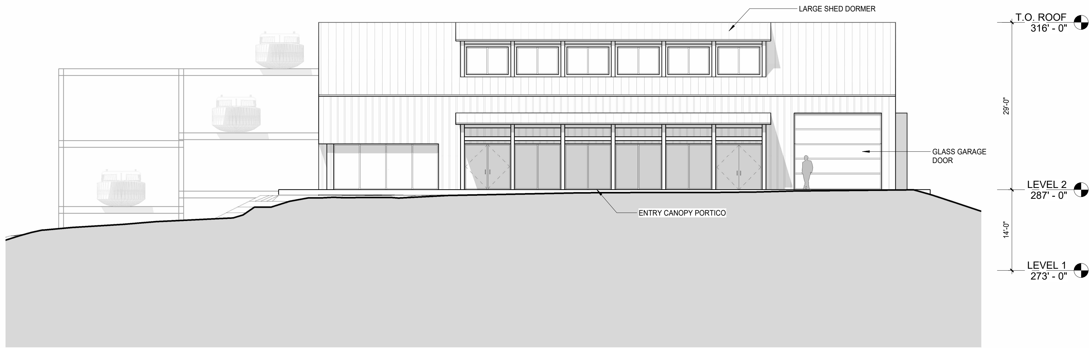
① Northeast Elevation 1" = 10'-0"
