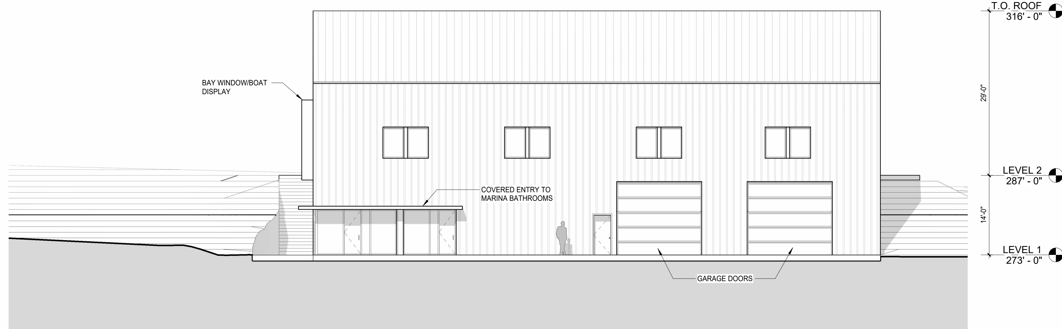
③ Southwest Elevation 1" = 10'-0"
