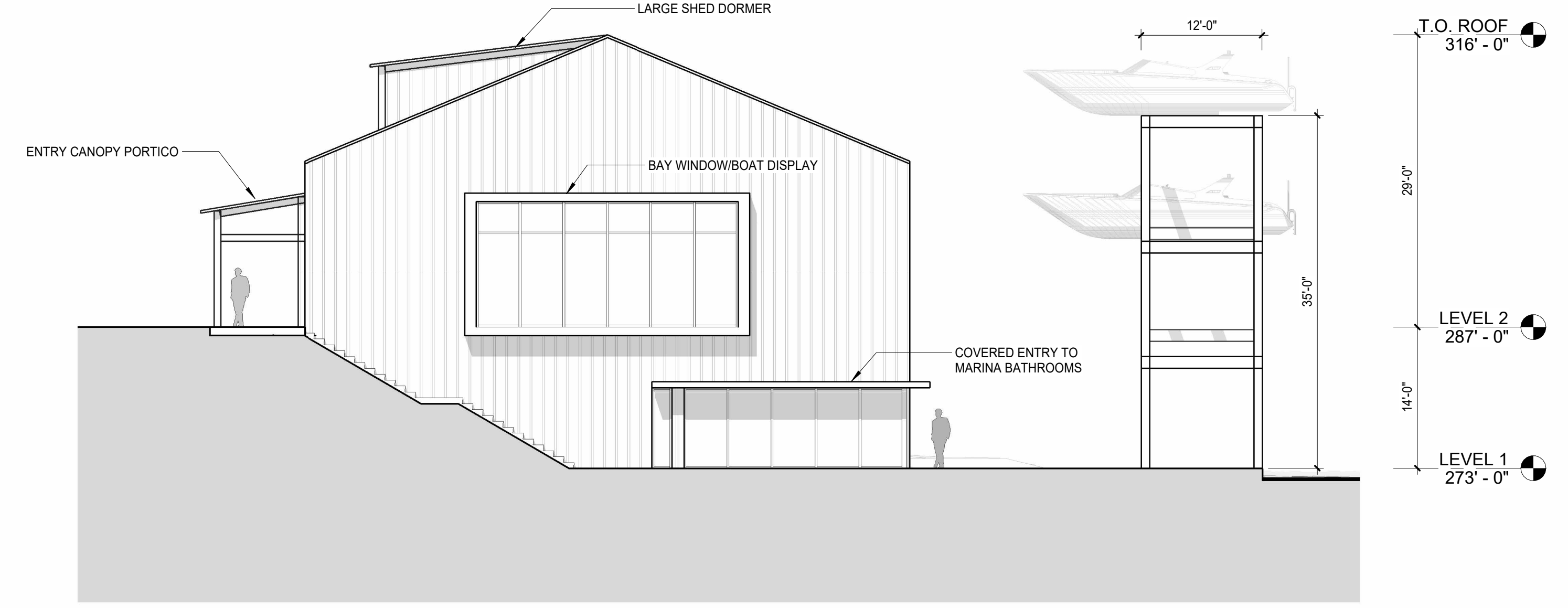
② Northwest Elevation 1" = 10'-0"
