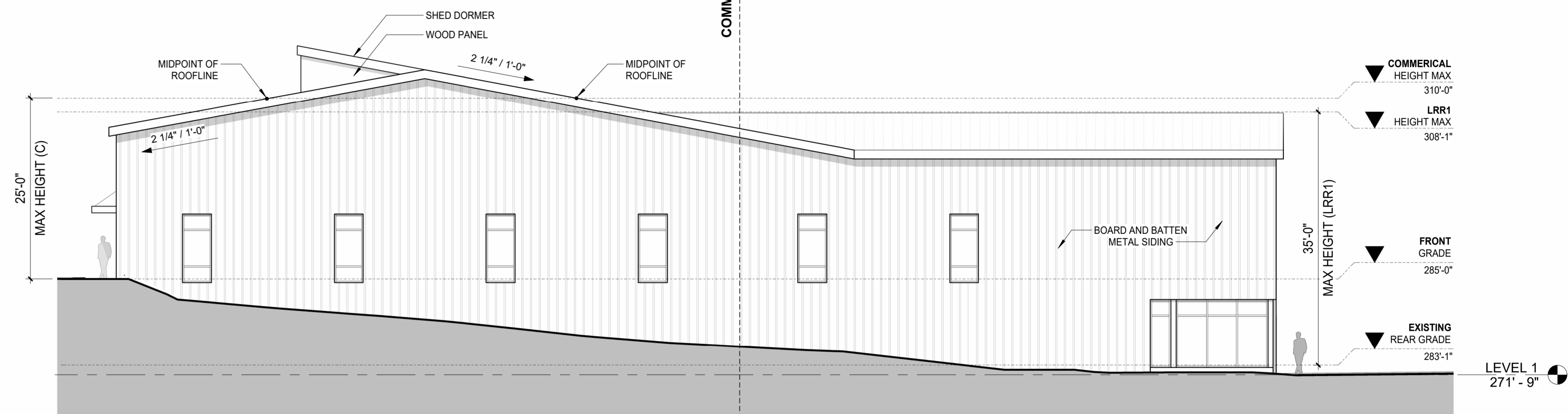
2 NORTHWEST ELEVATION 3/32" = 1'-0"
