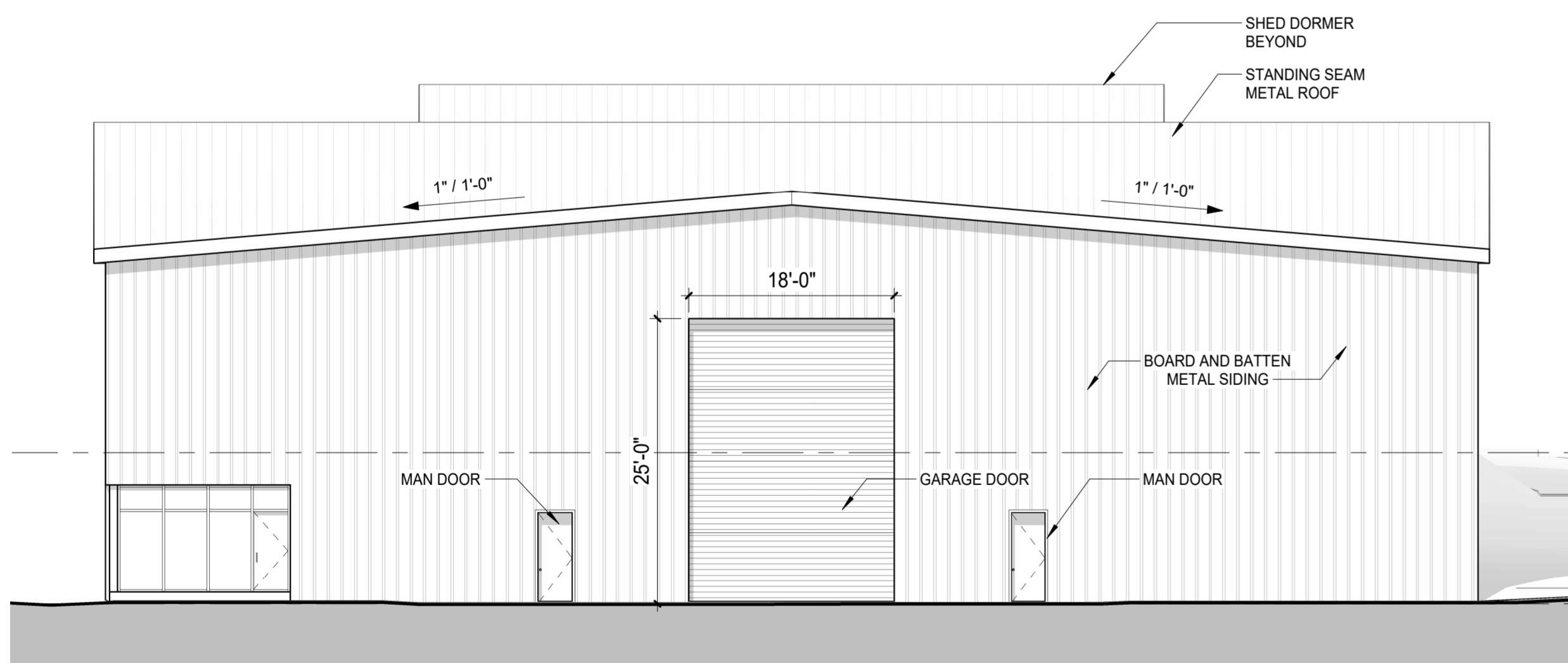
3 SOUTHWEST ELEVATION 3/32" = 1'-0"
